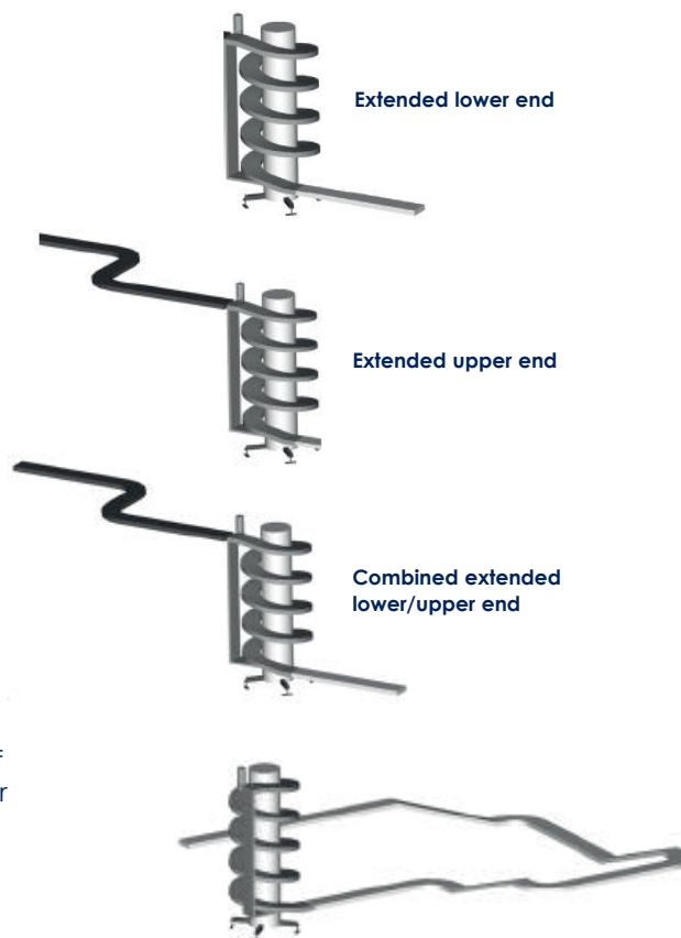
SpiralVeyor® combined with AmbaVeyor
